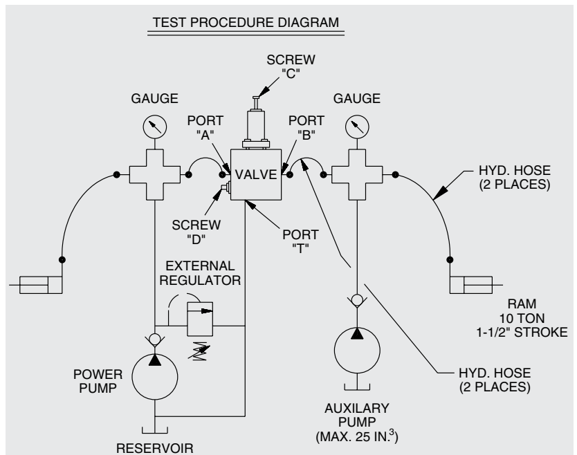
The diagram above is for hydraulic assembly test only and has nothing to do with customer setup.
