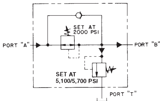
HYDRAULIC SCHEMATIC
